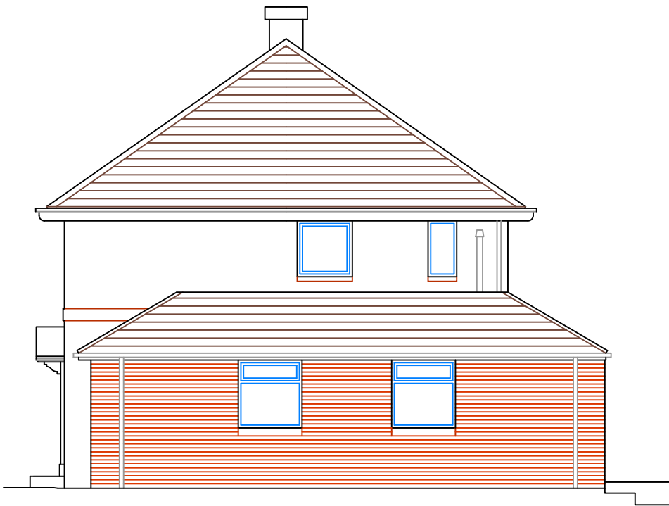
Side Elevation
