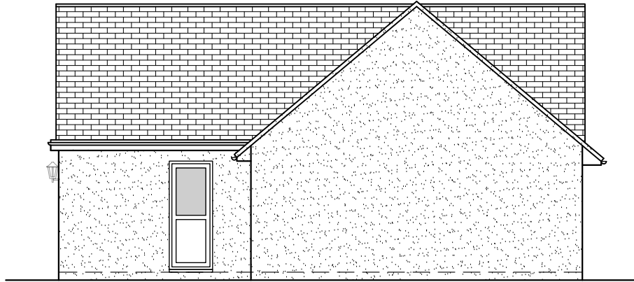
SOUTH Elevation
