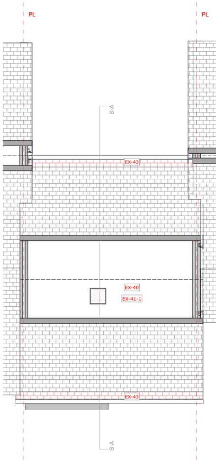
Proposed Eaves Level Plan
