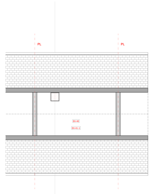
Proposed Eaves Level Plan
