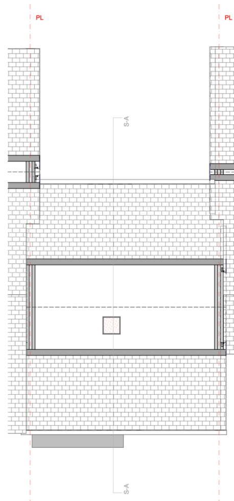
Existing Eaves Level Plan
