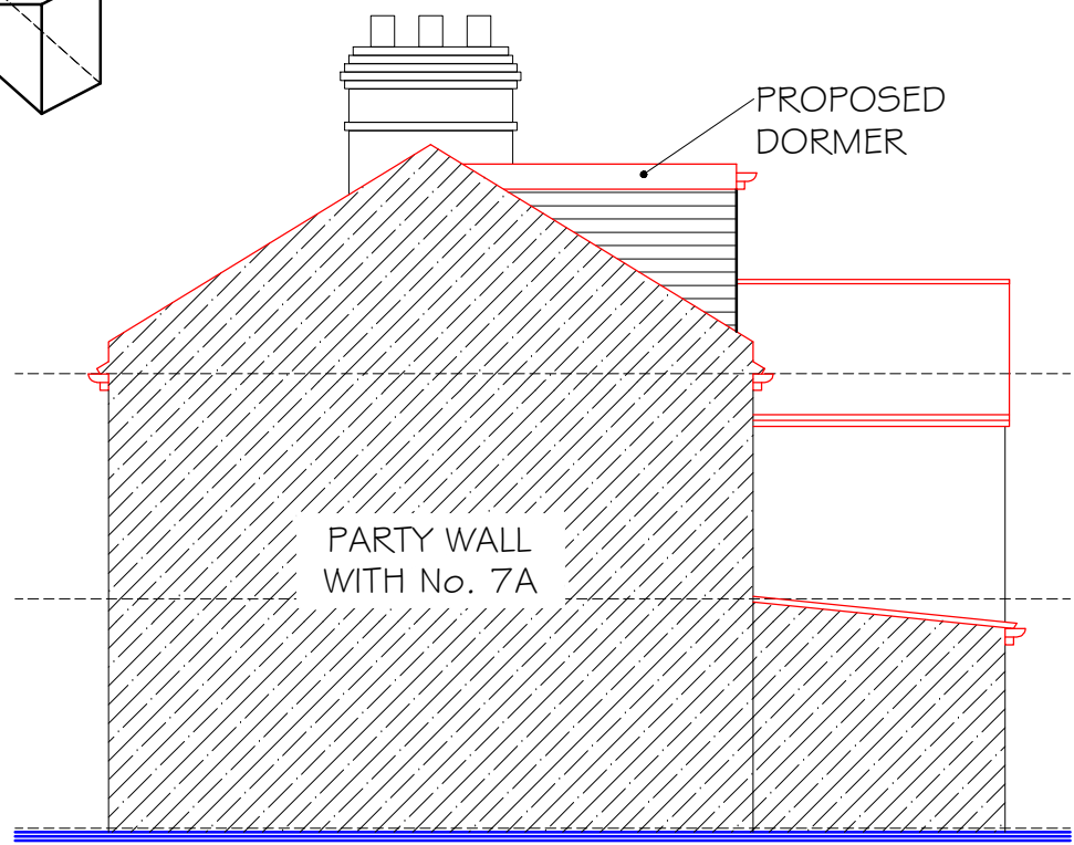
RIGHT HAND ELEVATION
