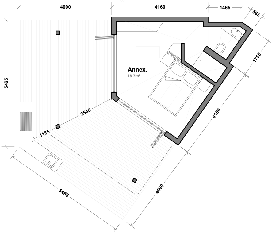
1 GROUND FLOOR PLAN SCALE - 1:100
