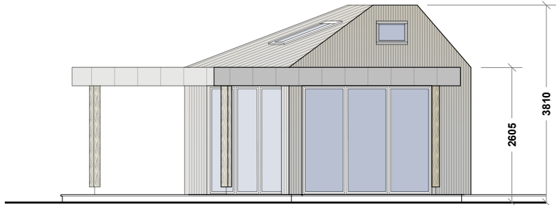
5 WESTERN ELEVATION SCALE - 1:100
