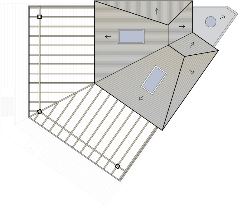
2 ROOF PLAN SCALE - 1:100
