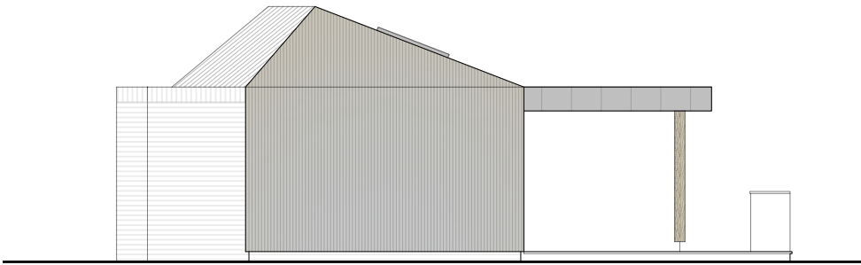
6 NORTHERN ELEVATION SCALE - 1:100
