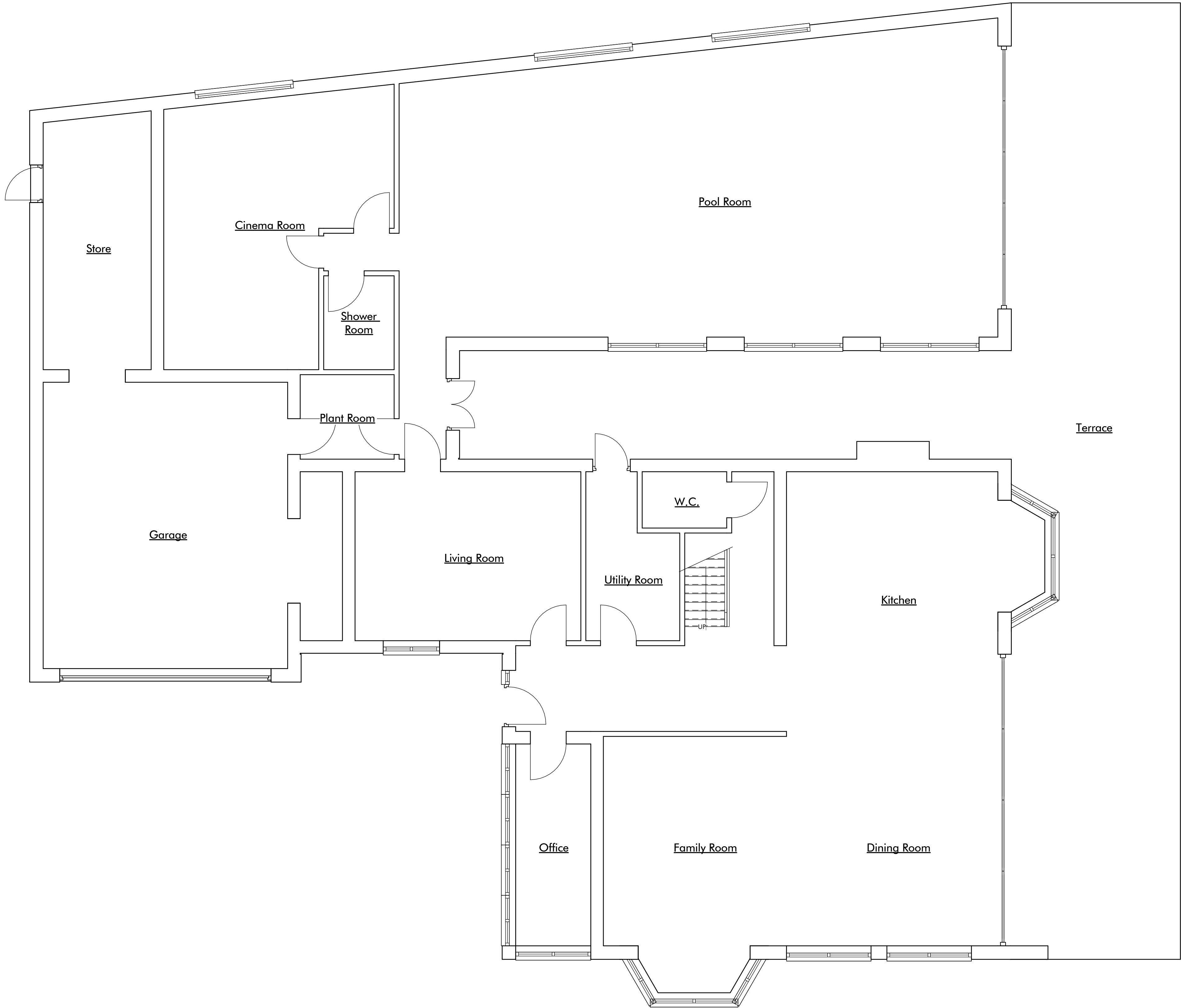
00 - Existing Ground Floor 1 : 50
