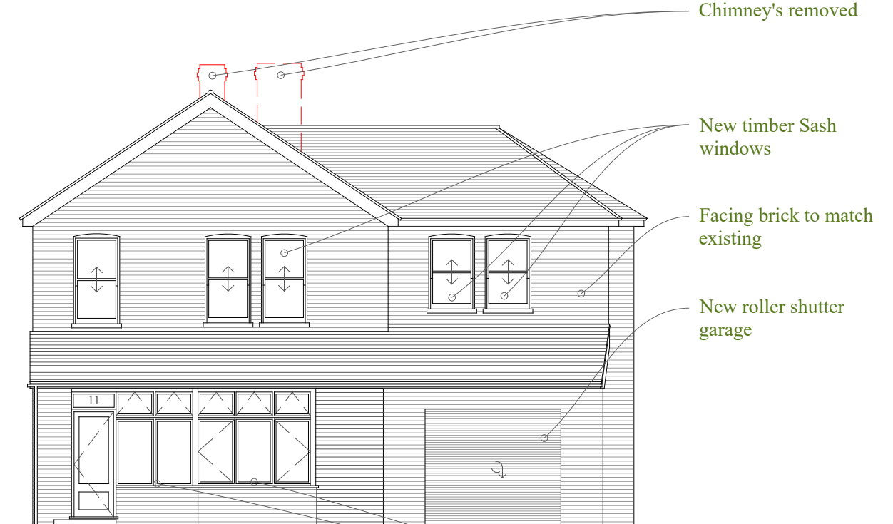
West 1:100 | PROPOSED
