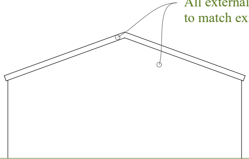
East 1:100 | PROPOSED
