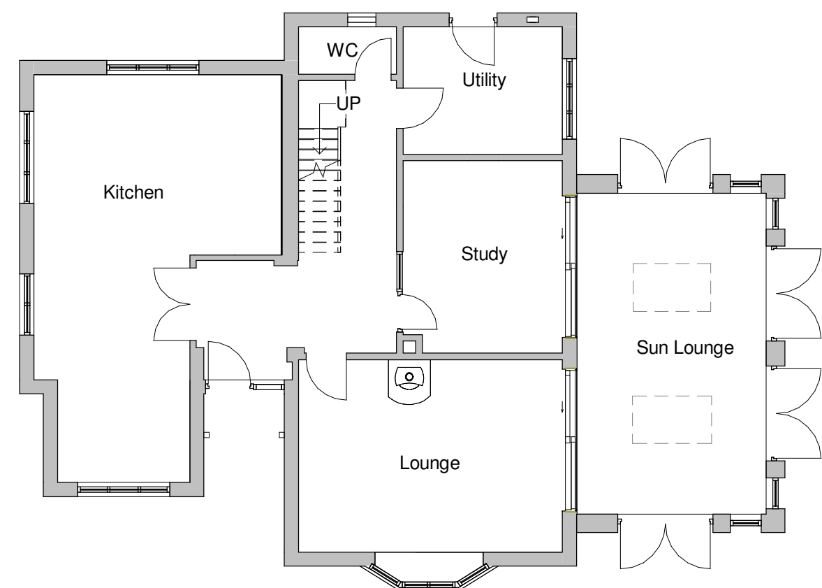
Proposed Ground Floor 1 : 100
