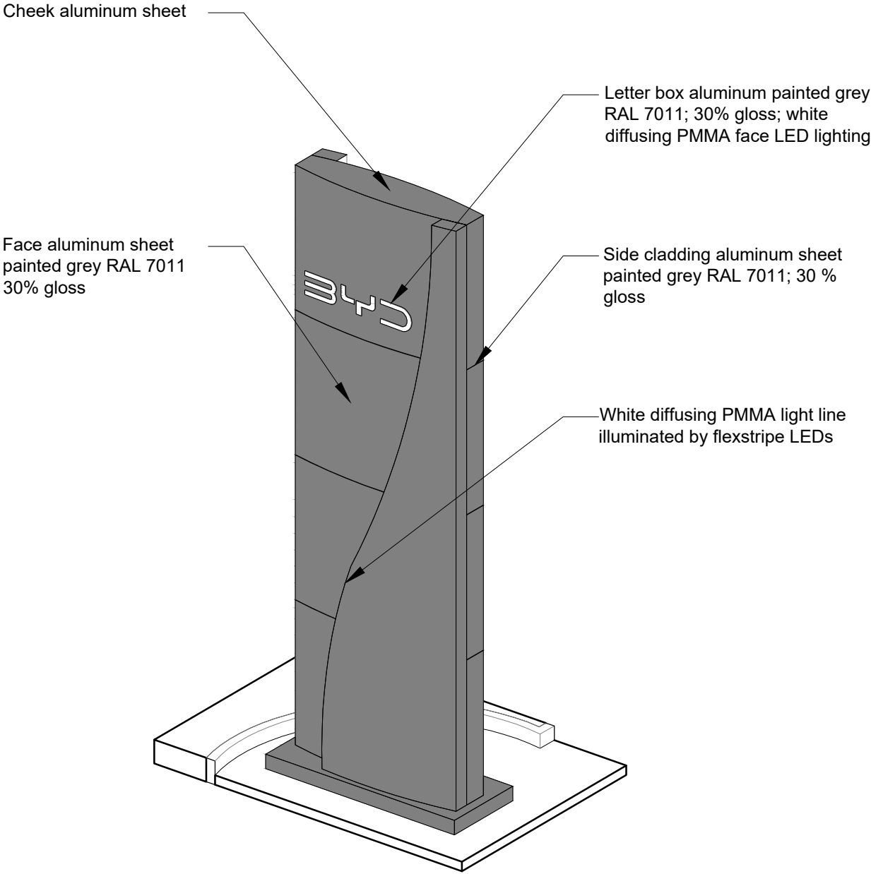
Totem Double Side - 3D View scale 1:50
