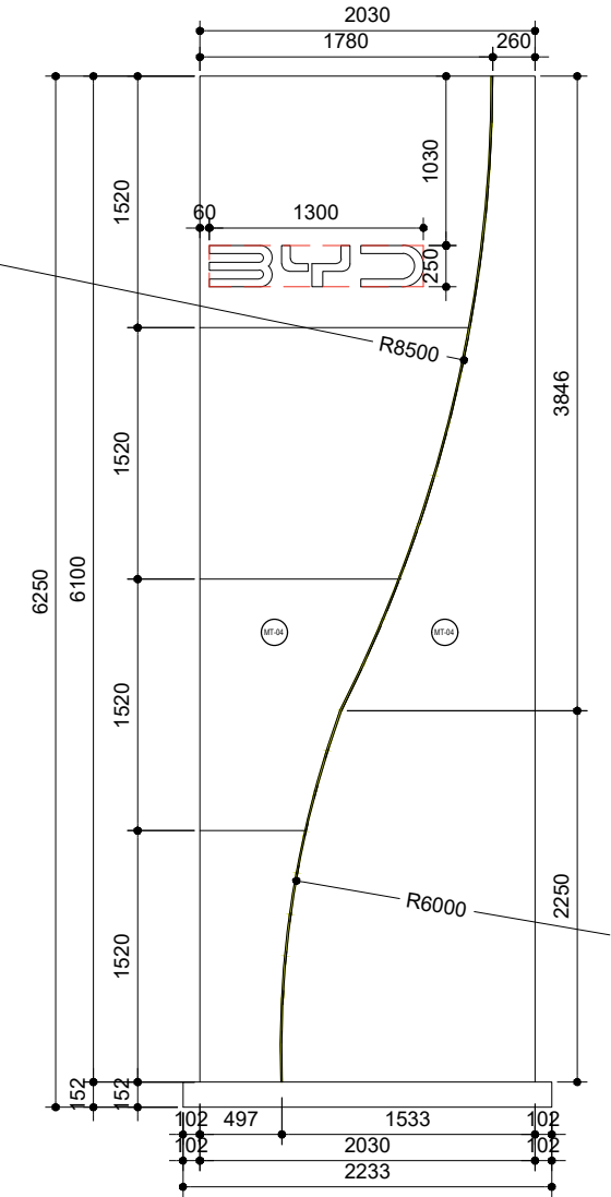
Totem Double Sided - Typical Elevation scale 1:50
