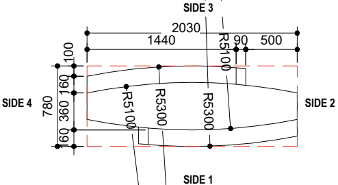
Totem Double Sided - Plan scale 1:50
