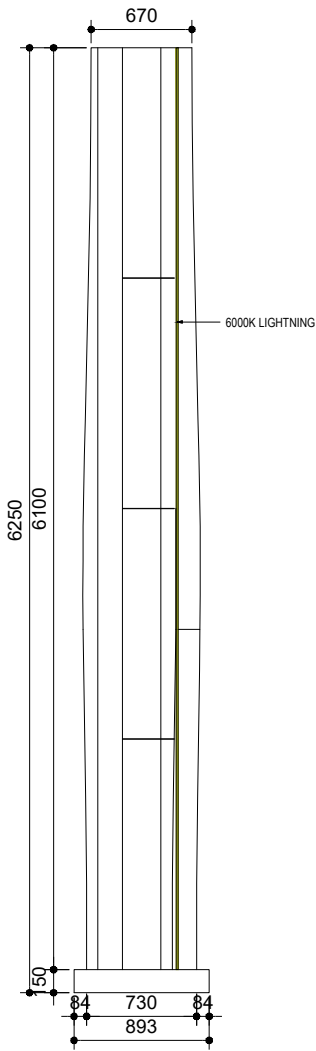
Totem Double Sided - Section scale 1:50
