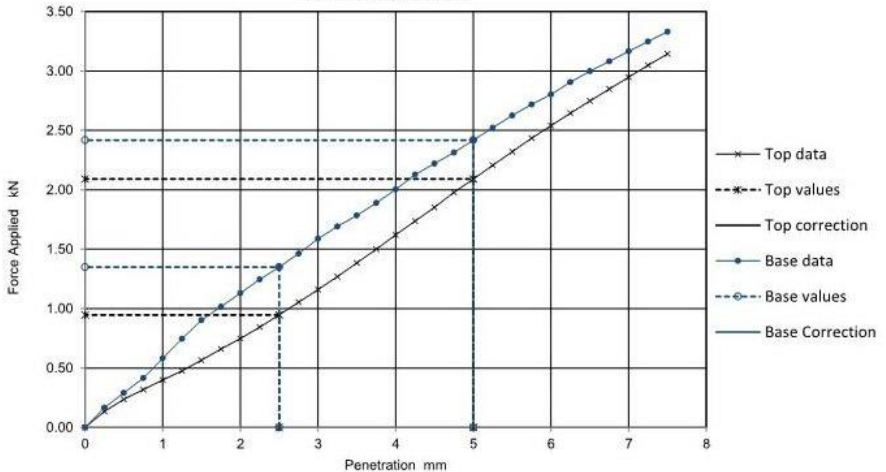
Force v Penetration Plots
