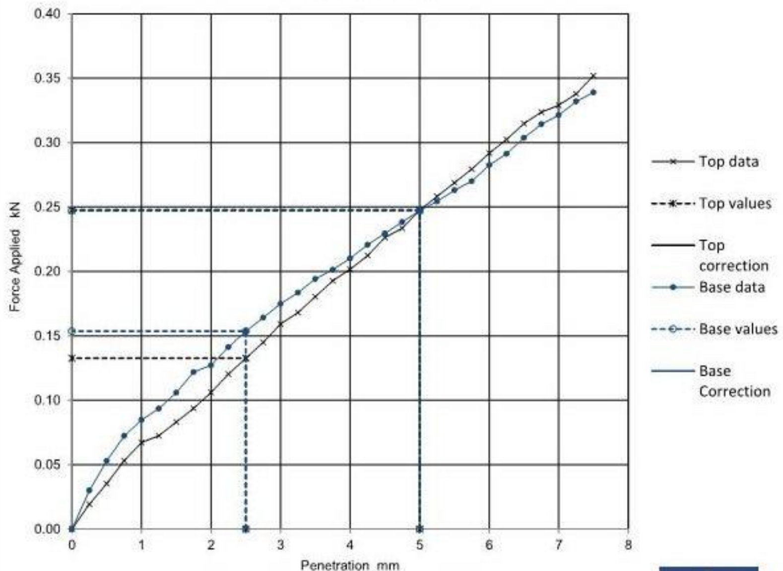
Force v Penetration Plots
