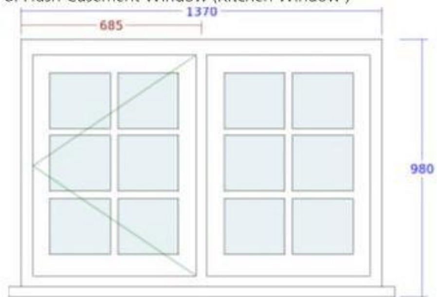
8. Flush Casement Window (Kitchen Window )
