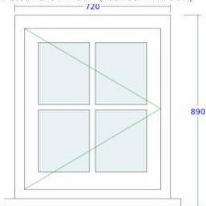
4. Flush Casement Window (Bathroom Window)
