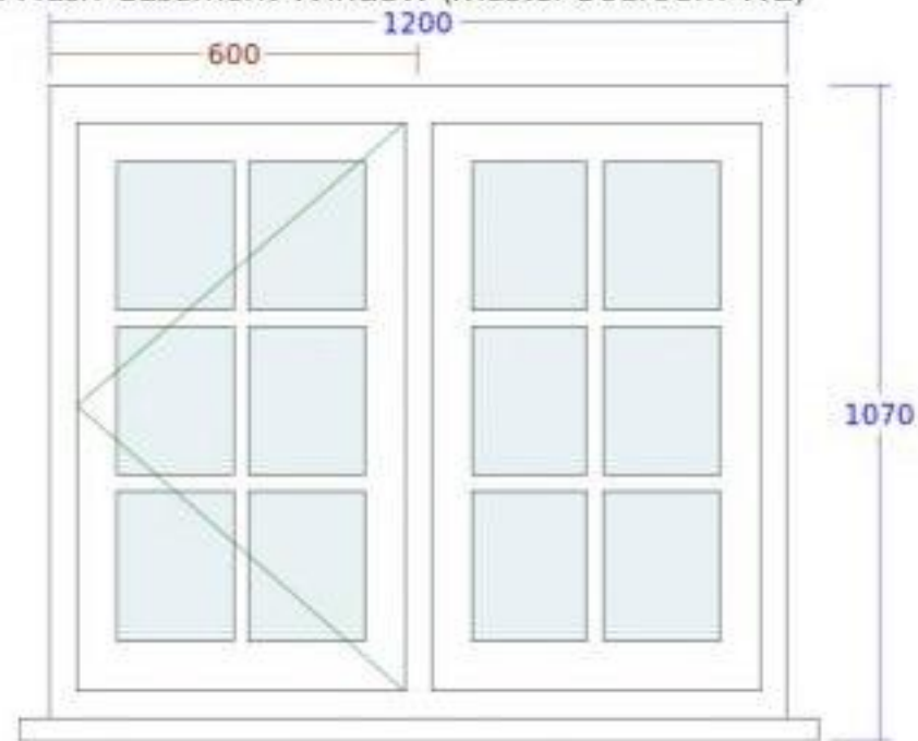
5. Flush Casement Window (Living Room Fixed )
