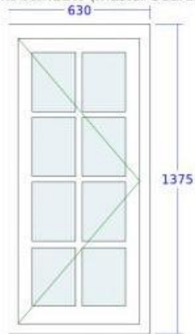
4. Flush Casement Window (Bathroom Window)
