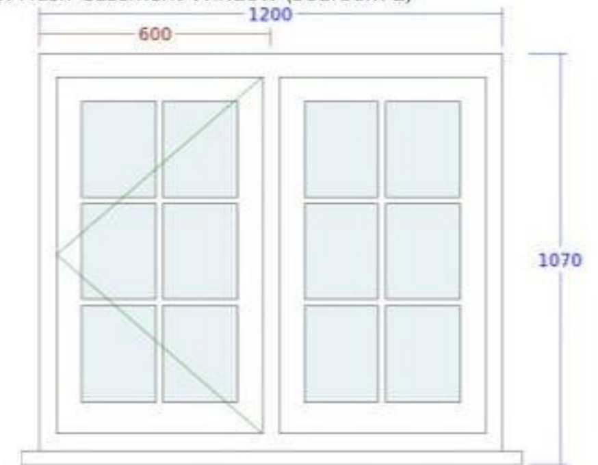
6. Flush Casement Window (Living Room W1)
