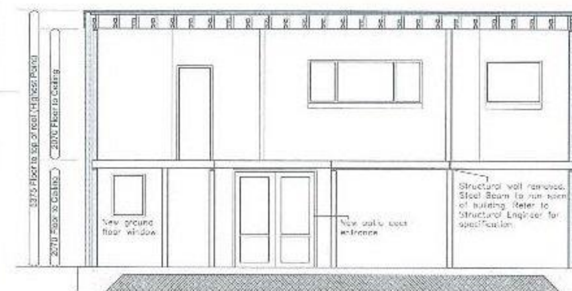
PROPOSED SECTION A-A SCALE 1:50 @A1
