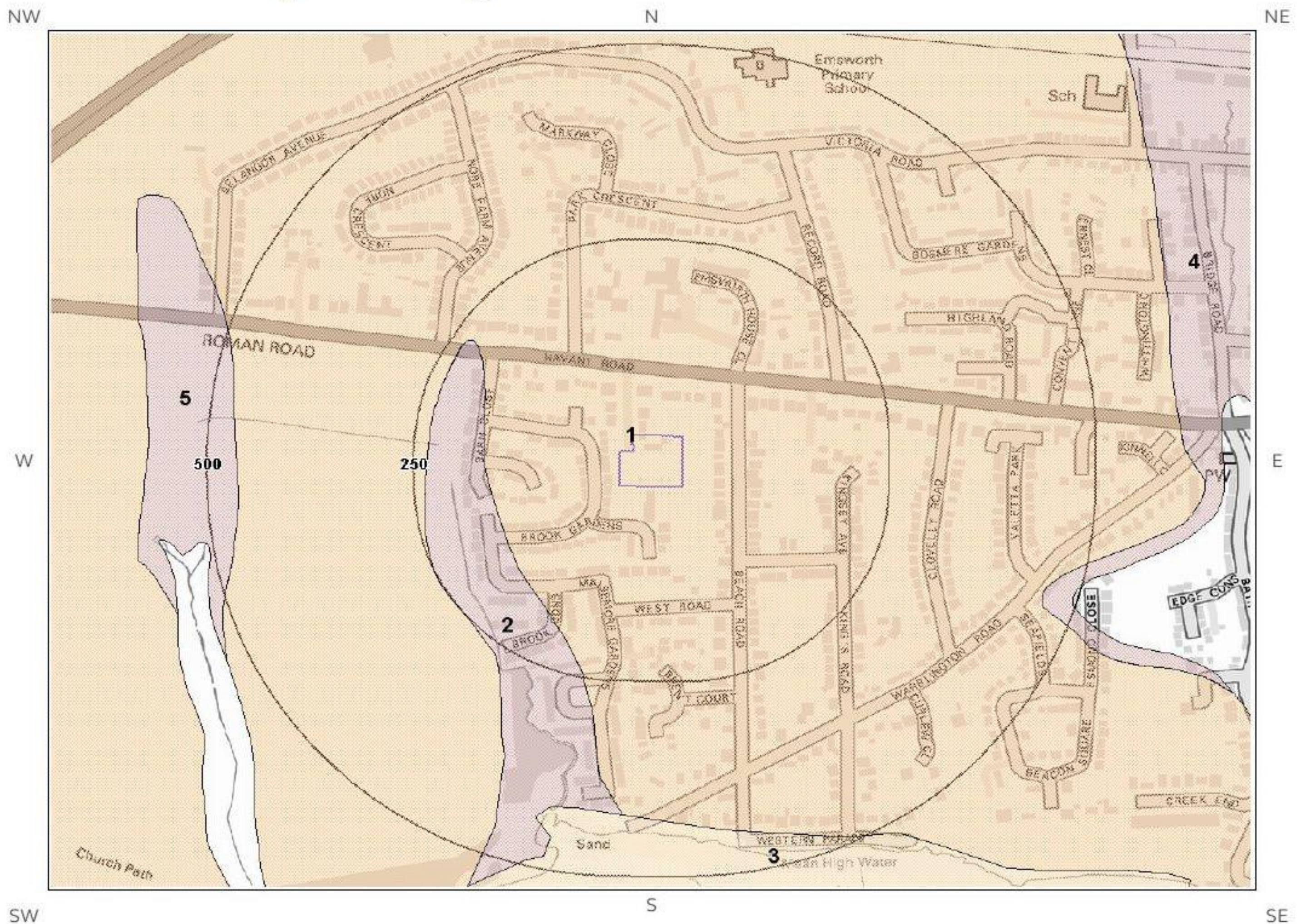
Superficial Deposits and Landslips Legend
