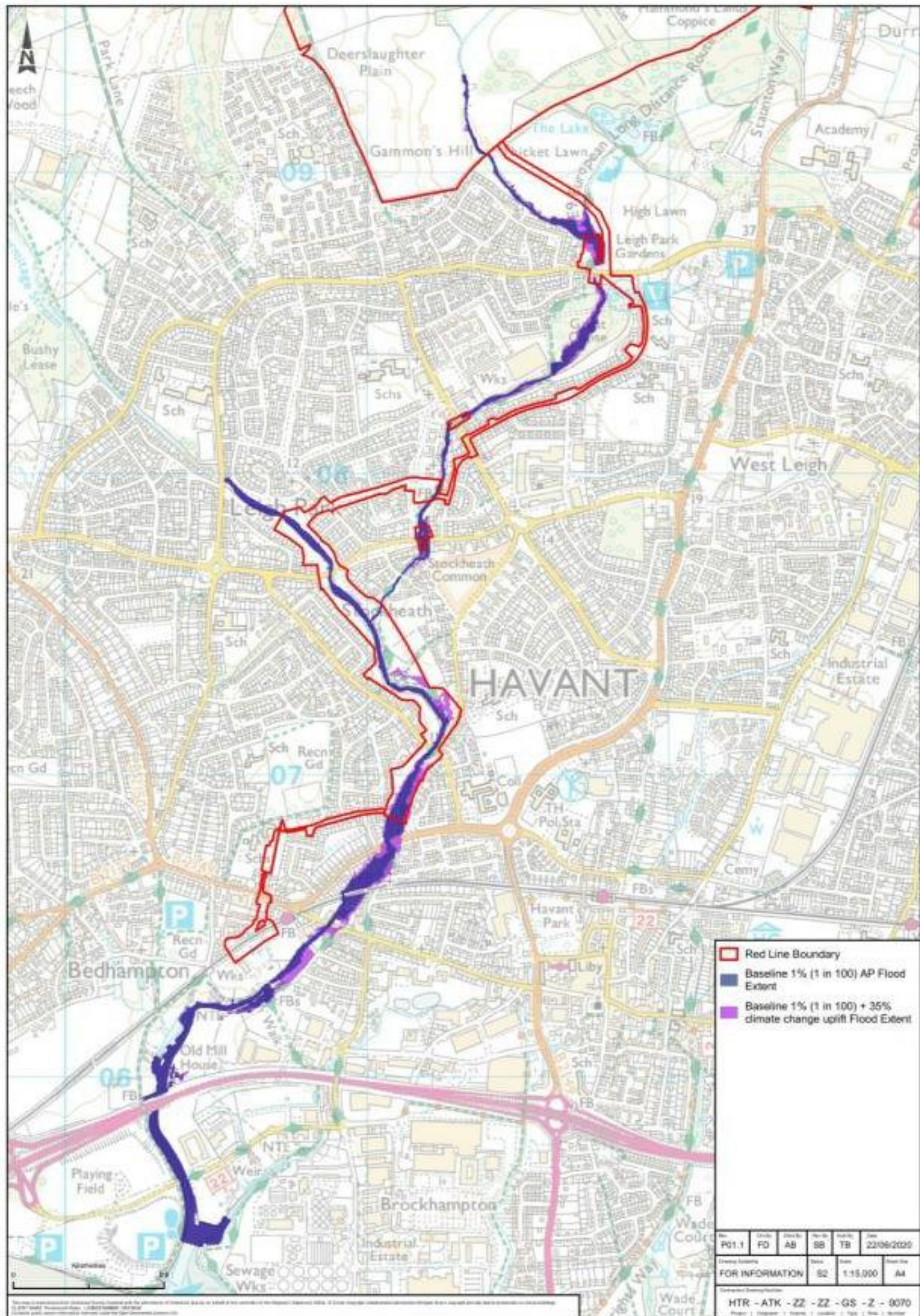
Figure 3-3 - Existing Flood Risk (Baseline 1 in 100 and 1 in 100 +cc)
