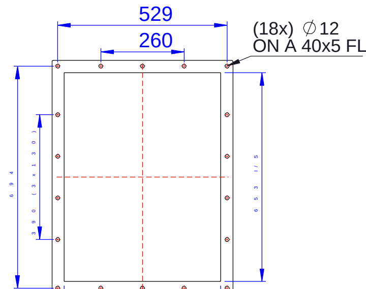
DISCHARGE FLANGE DETAIL
