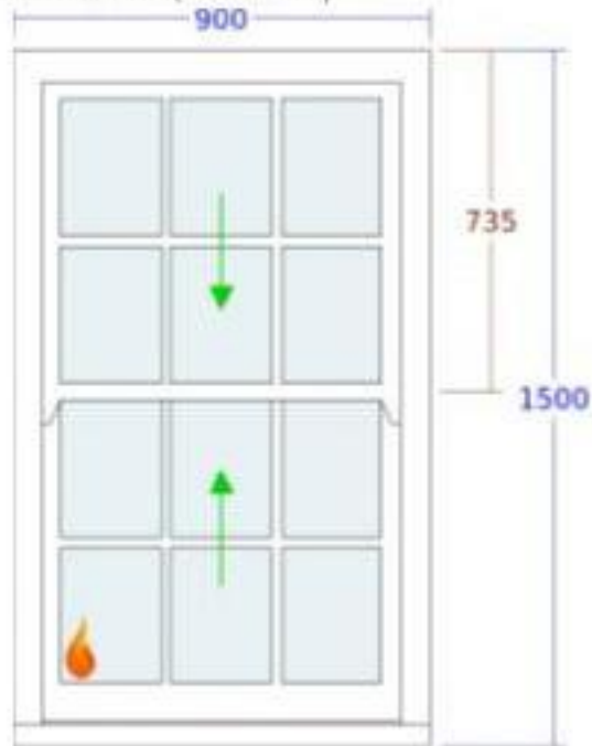
1. Slim Sash Window (Office 1 )
