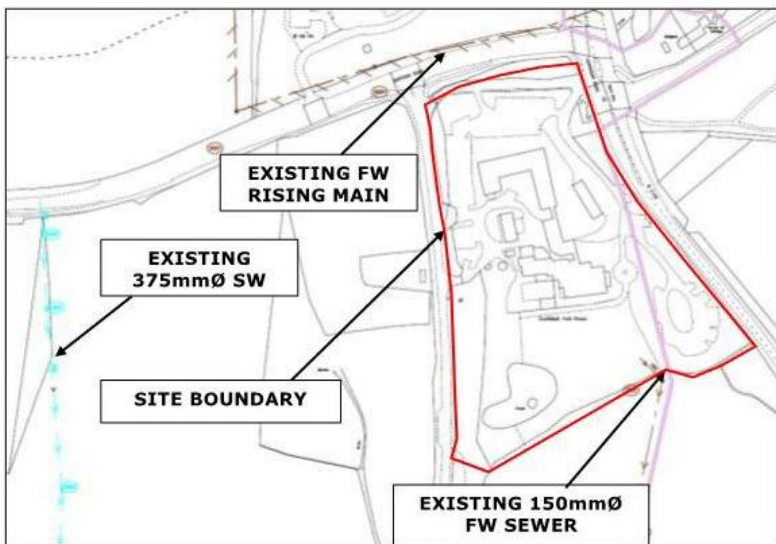
Figure 3-3: Southern Water Asset Plans (Extract)
