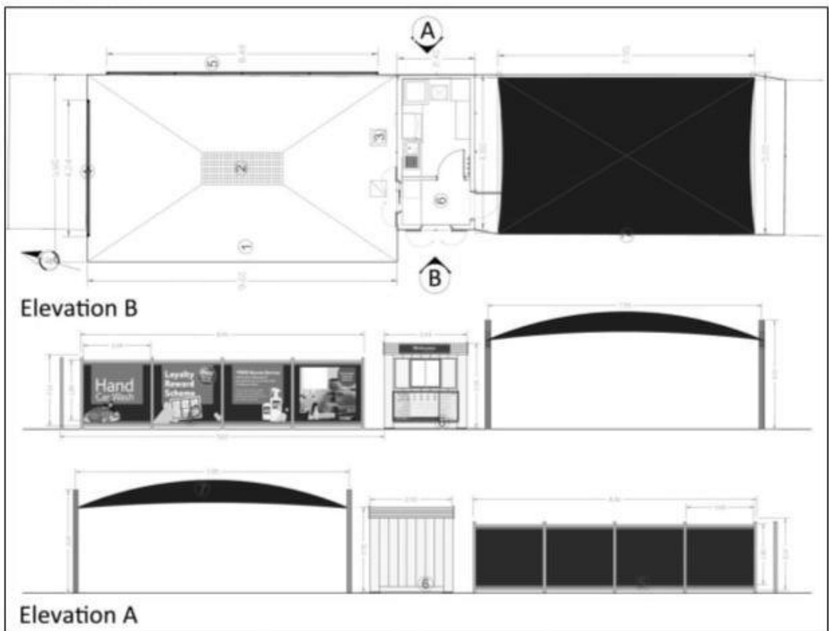
Figure 1 - Standard layout for a Waves car wash
