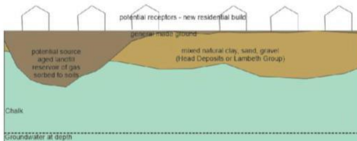
Figure 10: Simplistic ground model of western area of site
