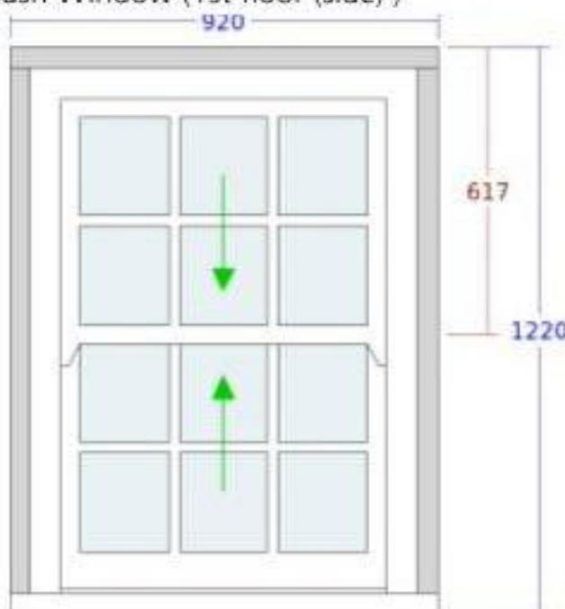
5. Slim Sash Window (1st floor (side) )
