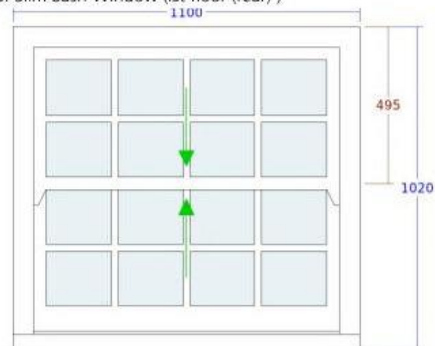
6. Slim Sash Window (1st floor (rear) )
