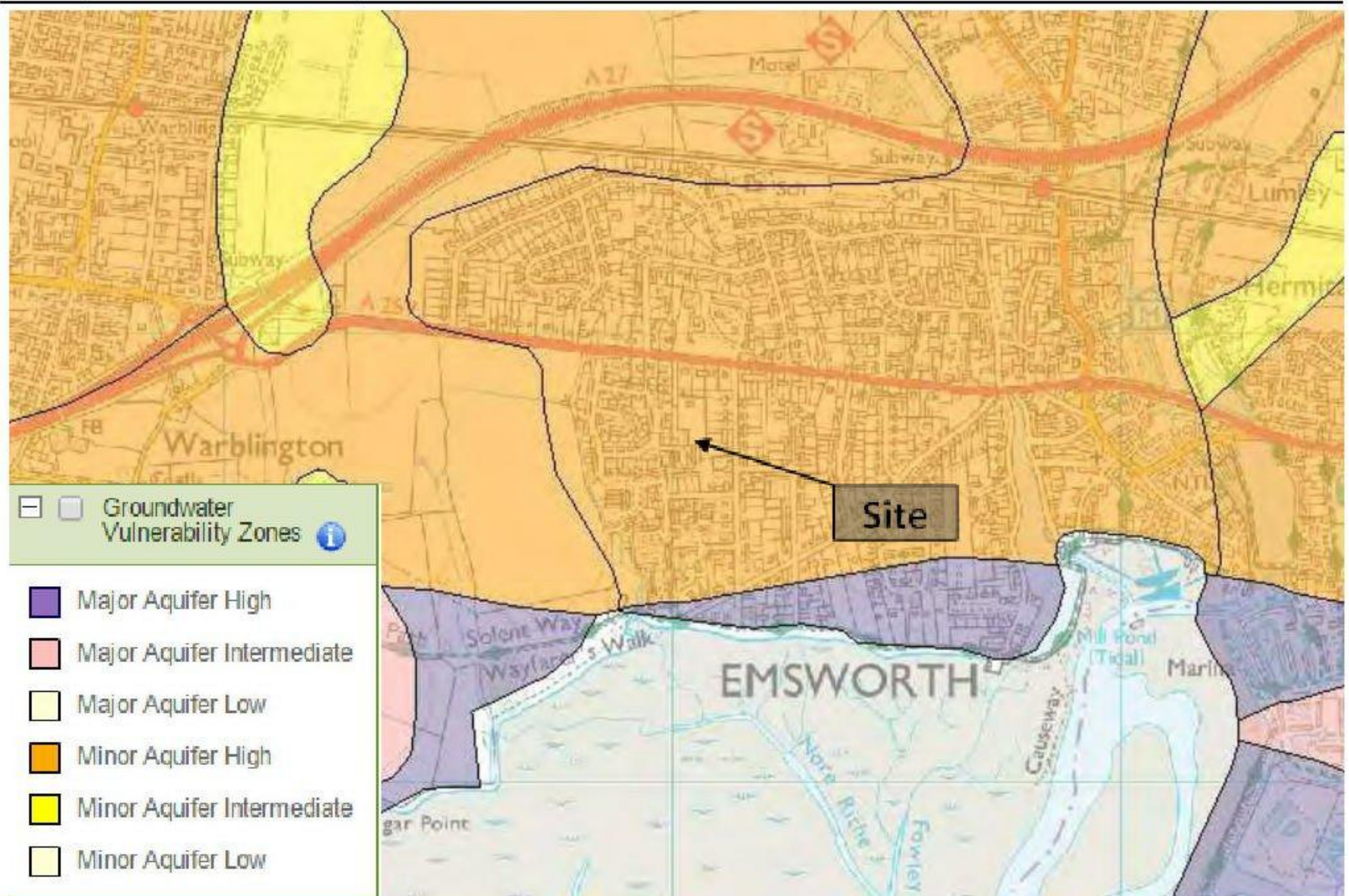
Groundwater Vulnerability Zones
