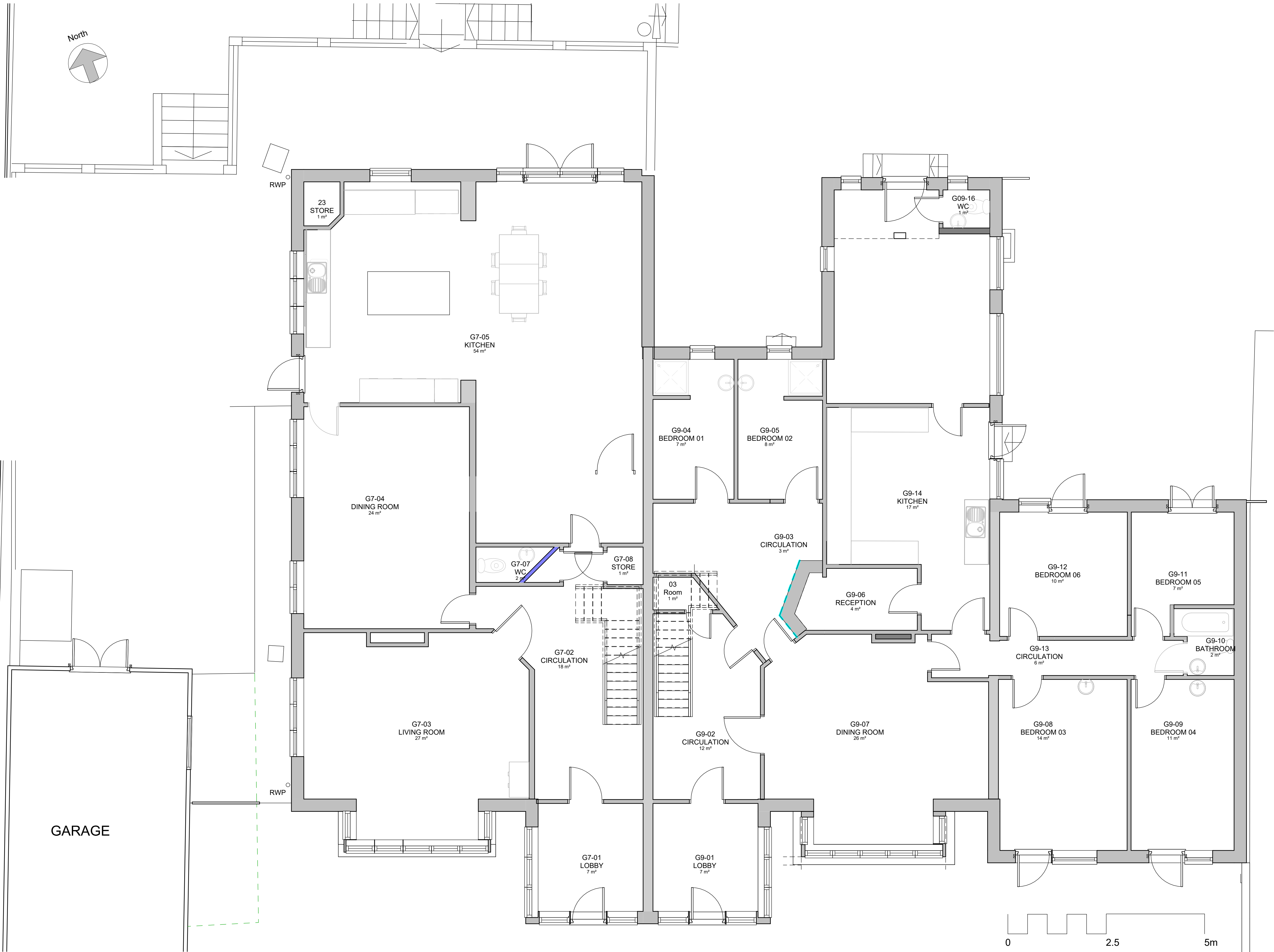
GROUND FLOOR AS EXISTING 1 : 50
