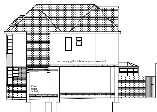
Proposed Section through extension
