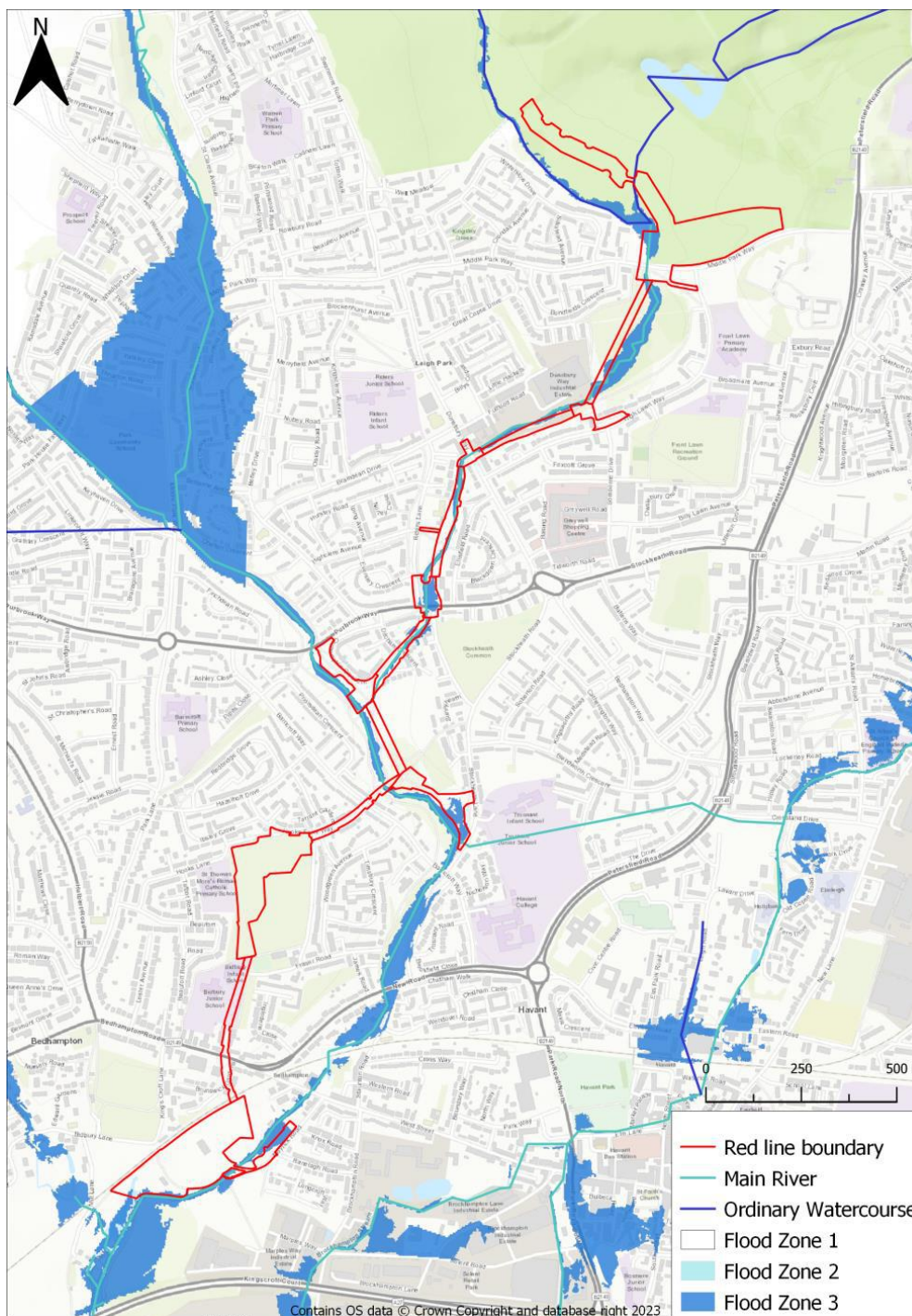
Figure 3.3 - Flood zones across the pipeline route
