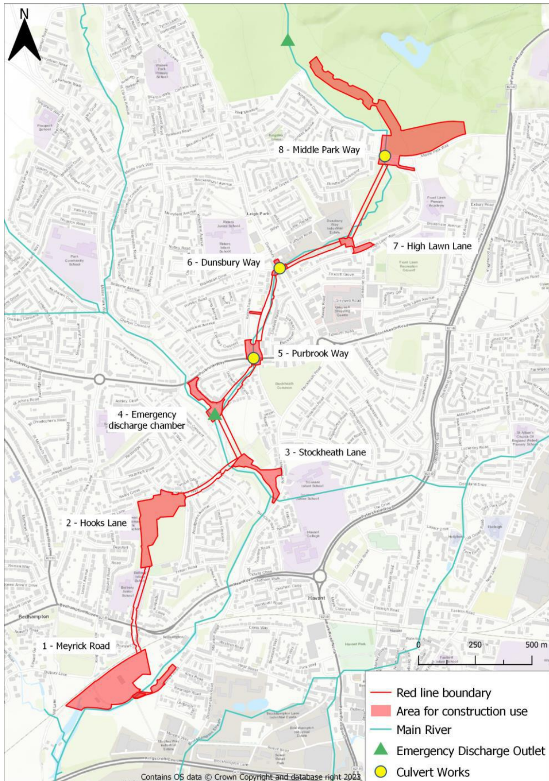
Figure 3.1 - Scheme Overview
