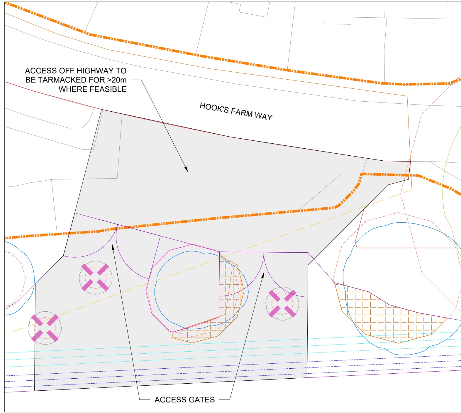
DETAIL A SCALE 1:200
