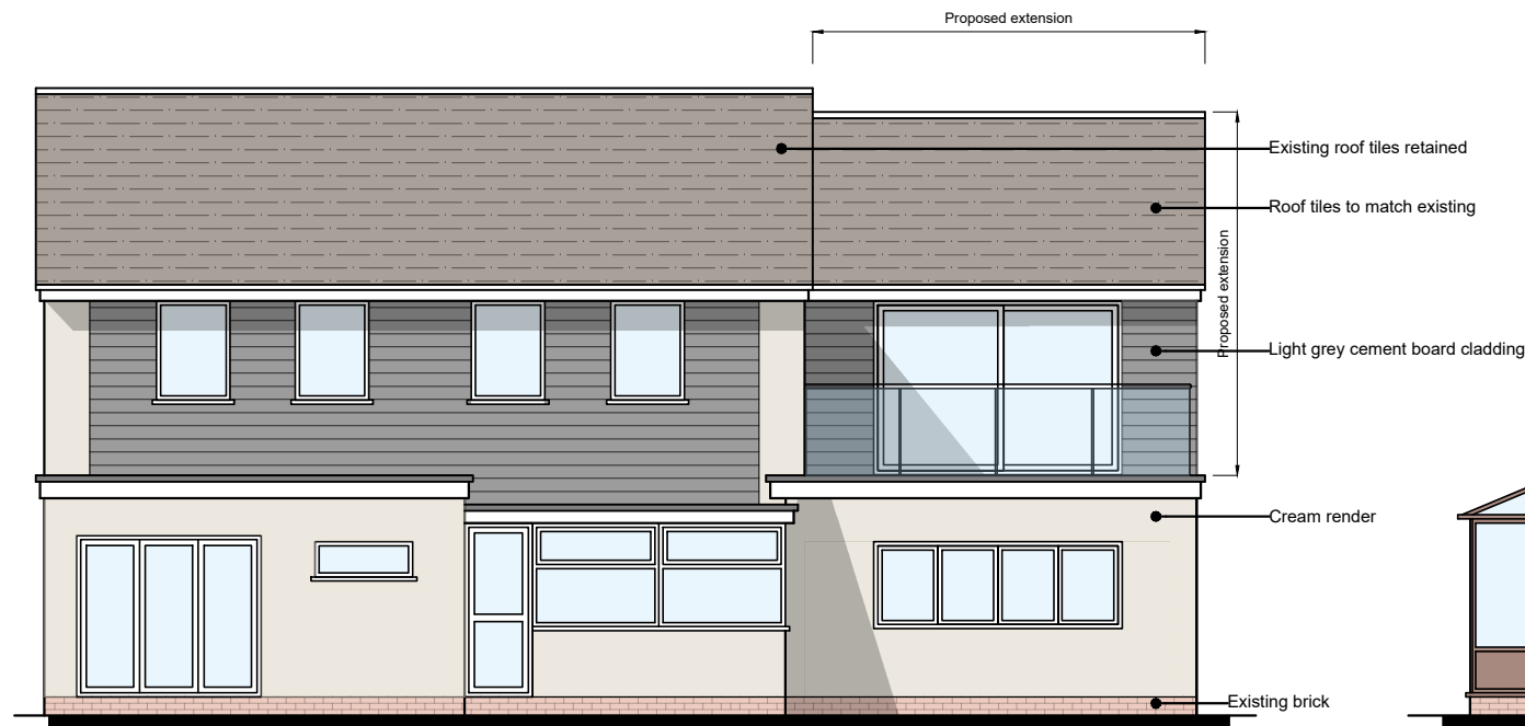
SOUTH Elevation
