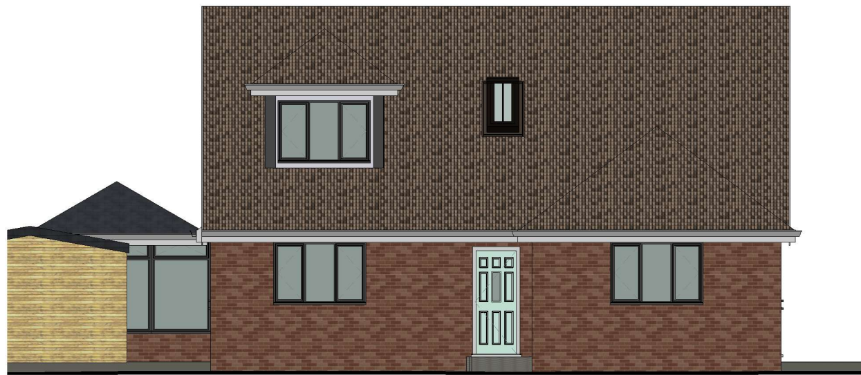
3 South Elevation 1 : 100
