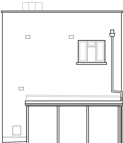
EXISTING NORTH-WEST ELEVATION
