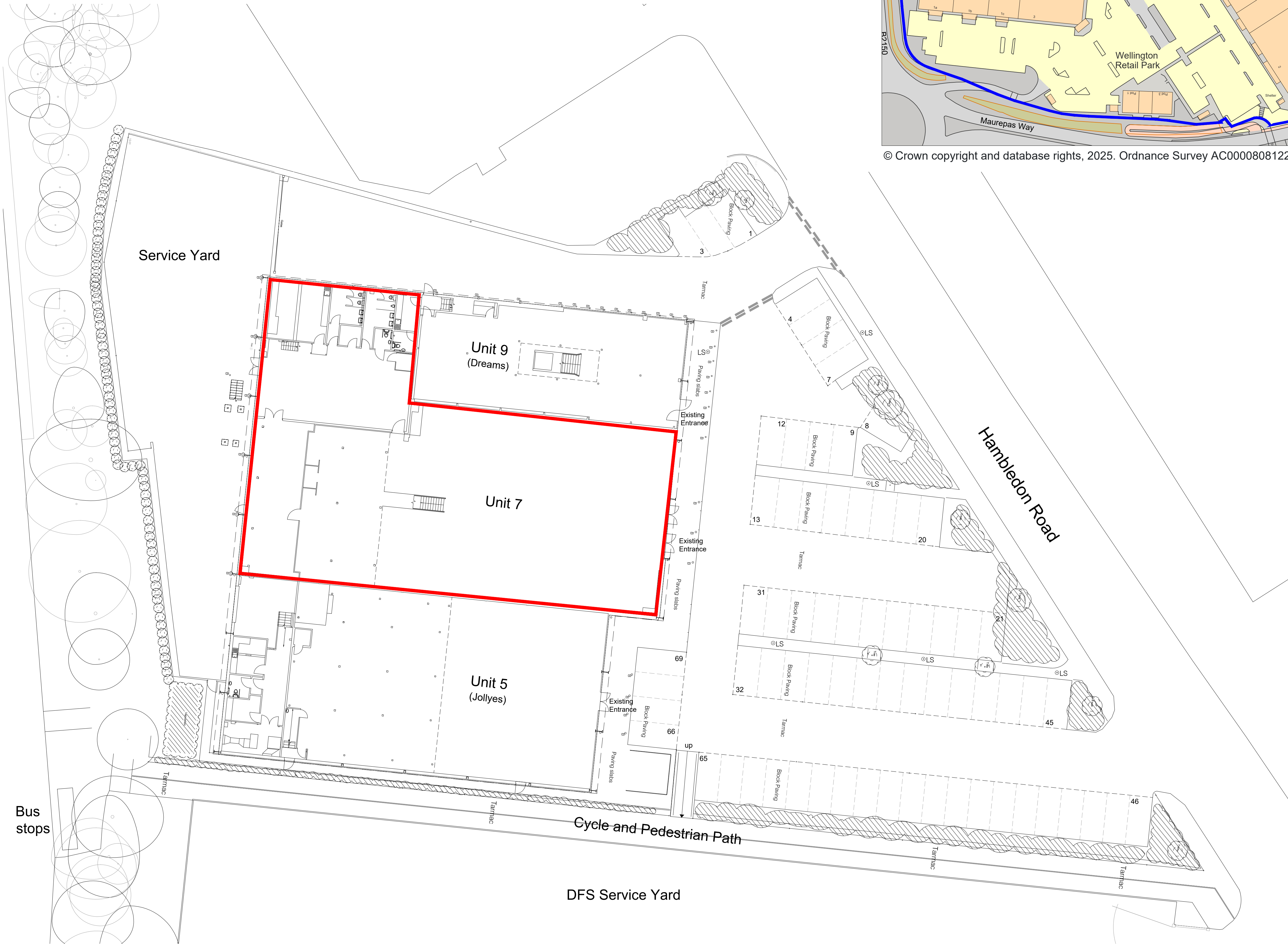
Existing Block Plan scale 1:200
