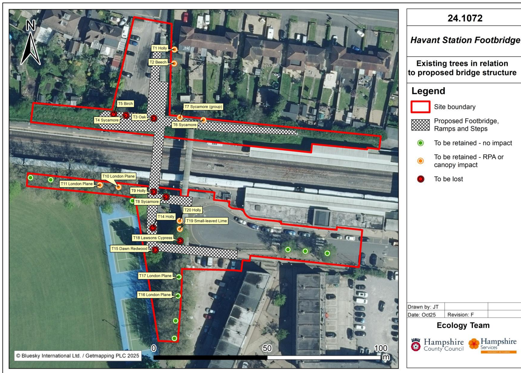
Figure A4.2 Existing tree plan in relation to proposed bridge structure (including trees outside redline boundary).
