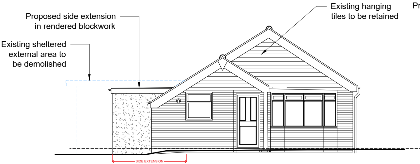
36 Selsmore Road NORTH ELEVATION
