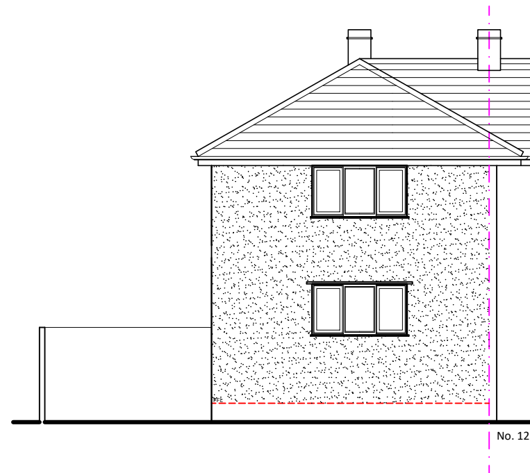
Existing south (front) elevation
