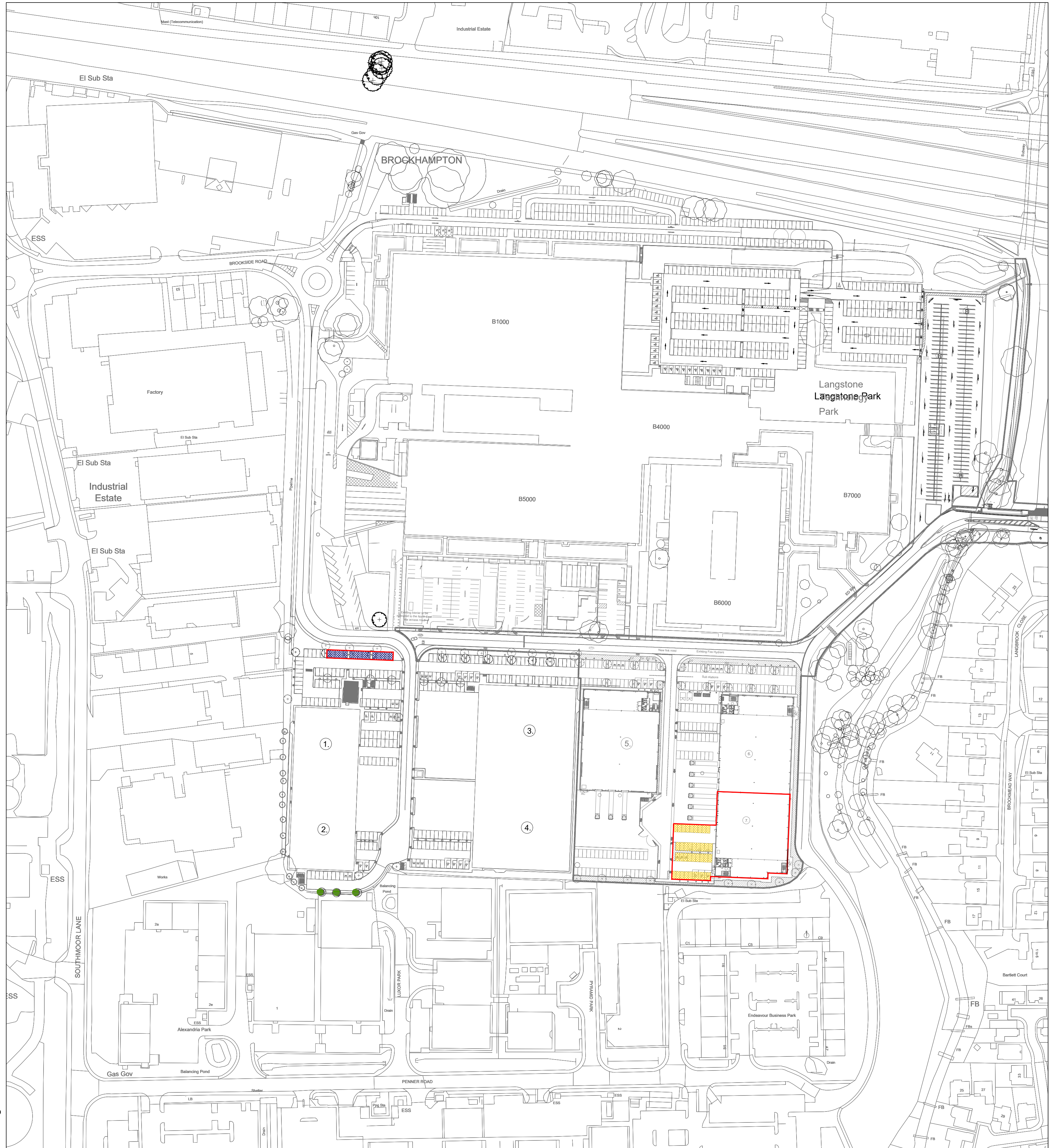
Location plan indicating parking (yellow hatched spaces) scale 1:1250
