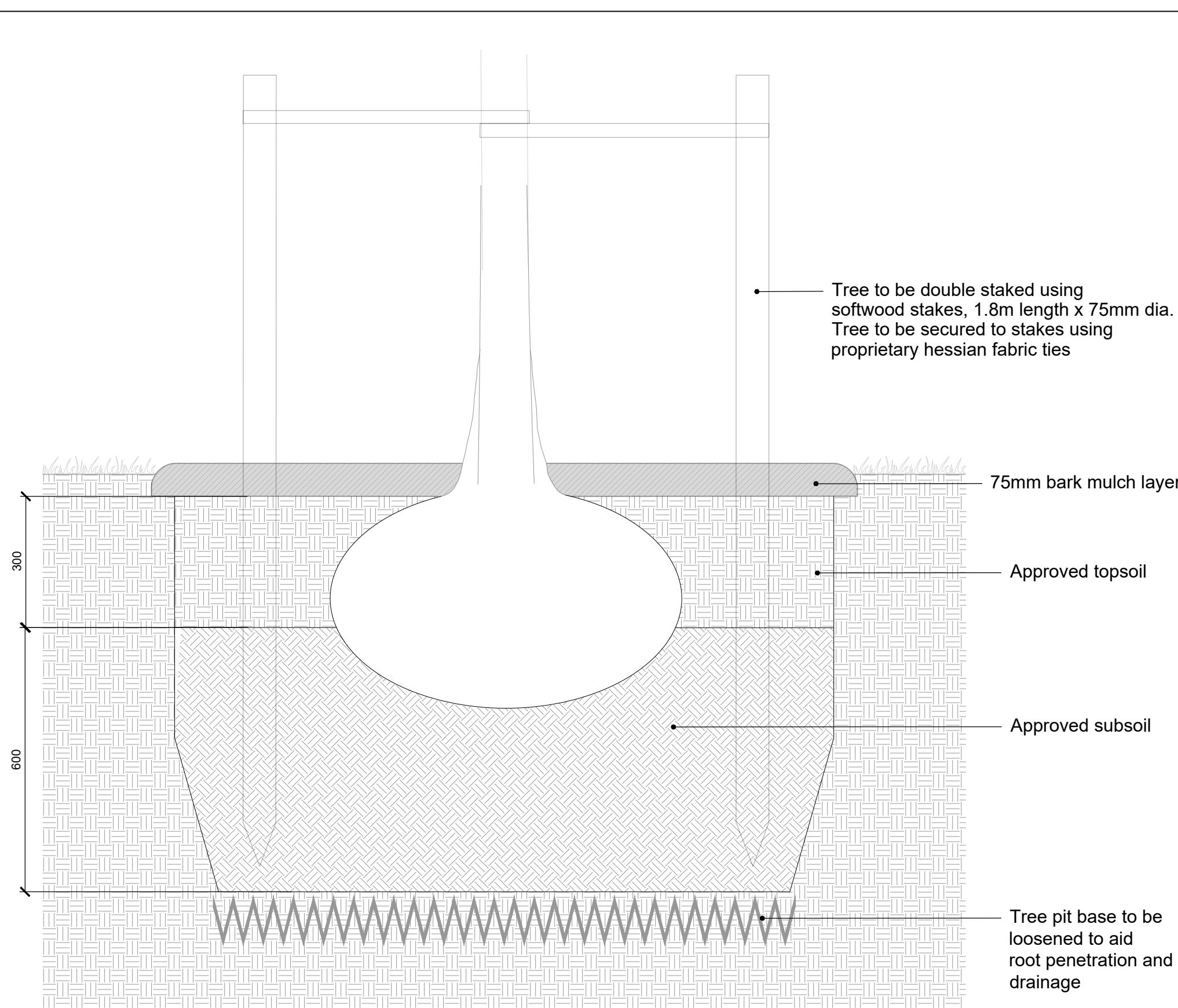
3 Standard Tree Pit- Typical Detail
