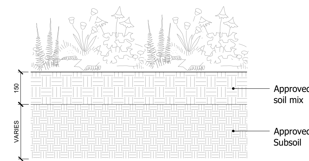
4 Scrub & Hedge Planting - Typical Detail
