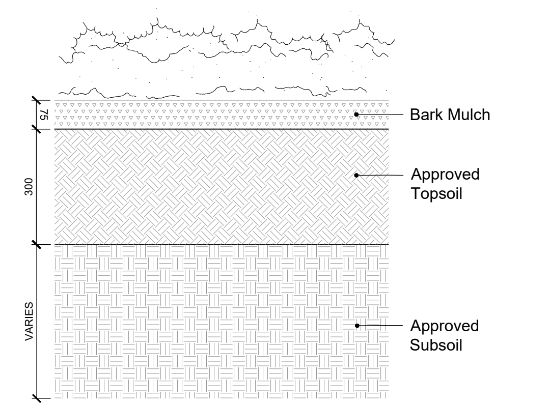
4 Scrub & Hedge Planting - Typical Detail
