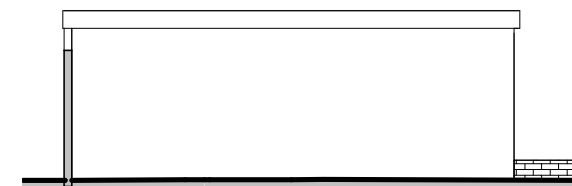
4 South Garage Elevation 1 : 100
