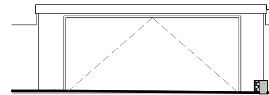
2 East Garage Elevation 1 : 100
