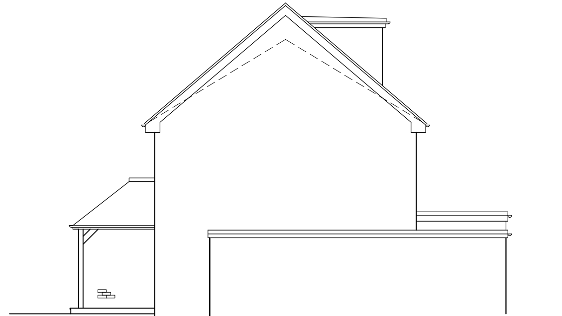
EAST: PROPOSED 1:100
