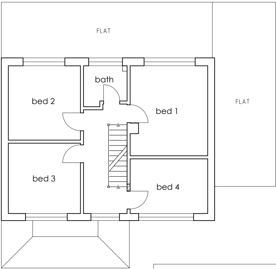
FIRST FLOOR: PROPOSED 1:100
