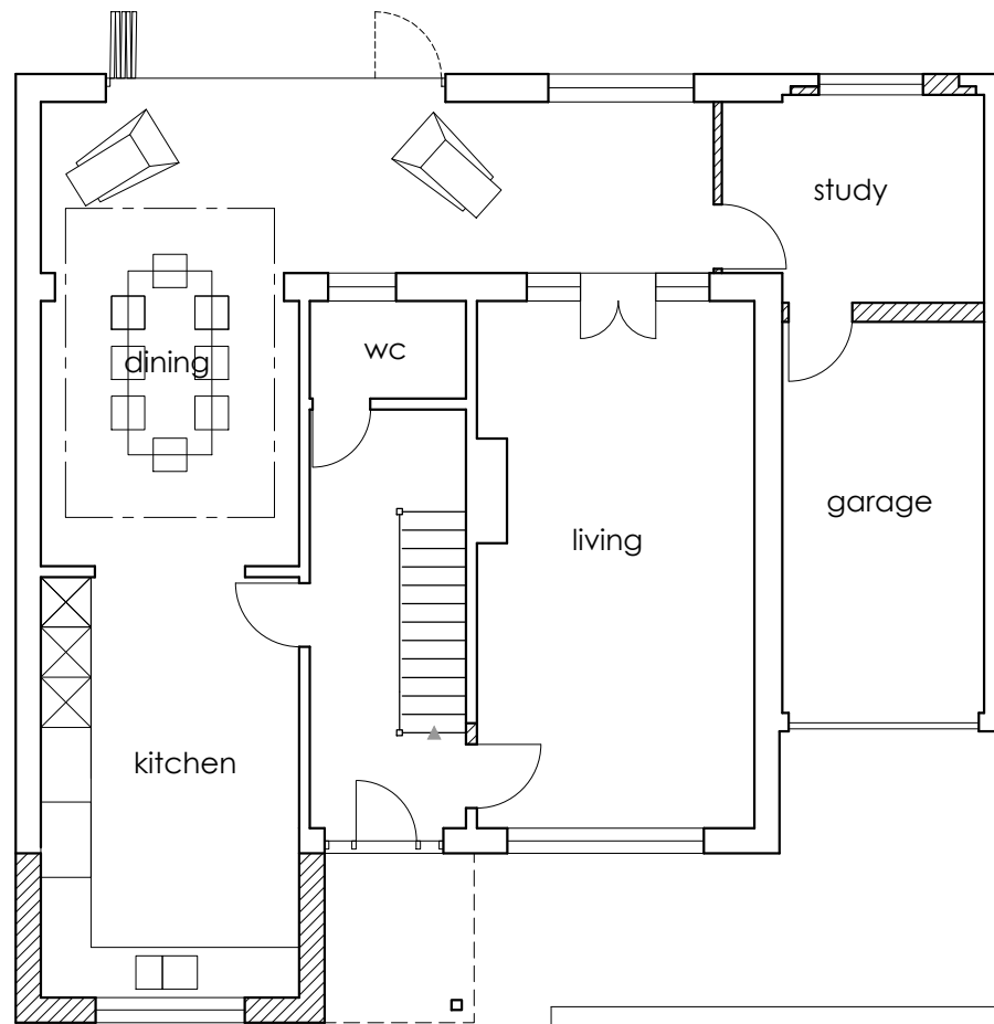
GROUND FLOOR: PROPOSED 1:100
