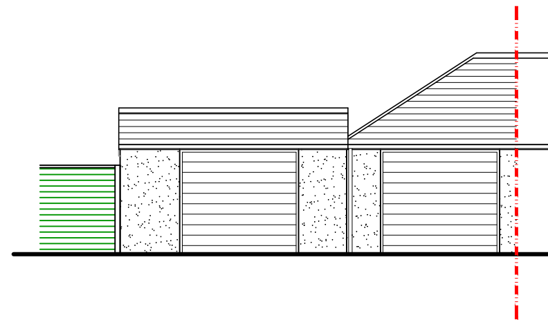
Front (west) elevation
