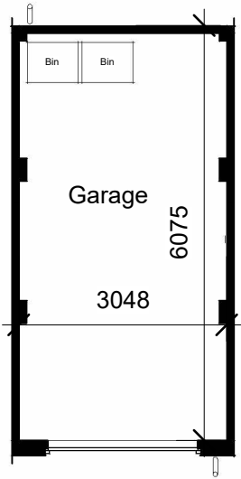
Level 00-Ground Floor 1 : 100
