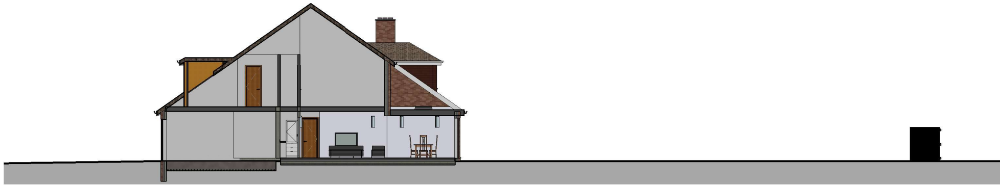
1 North South Site Section 1 : 200
