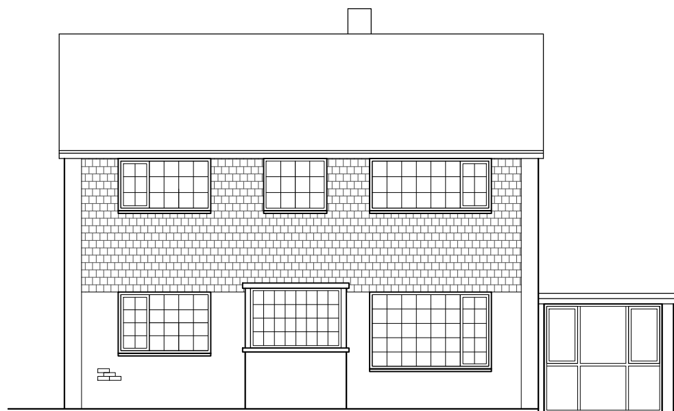
SOUTH: EXISTING 1:100
