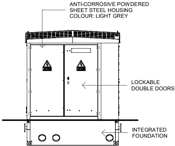
REAR ELEVATION 1:50
