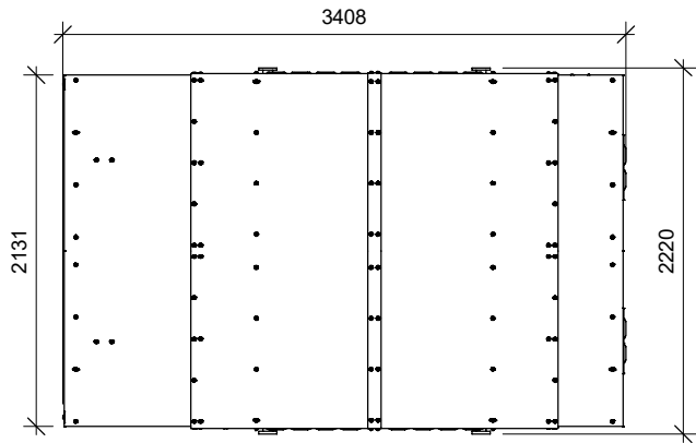
PROPOSED PLAN 1:50
