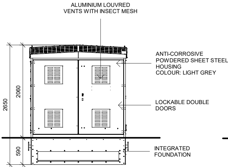
FRONT ELEVATION 1:50
