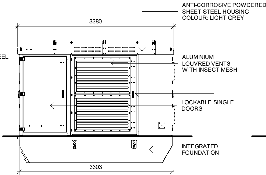
SIDE ELEVATION 1:50
