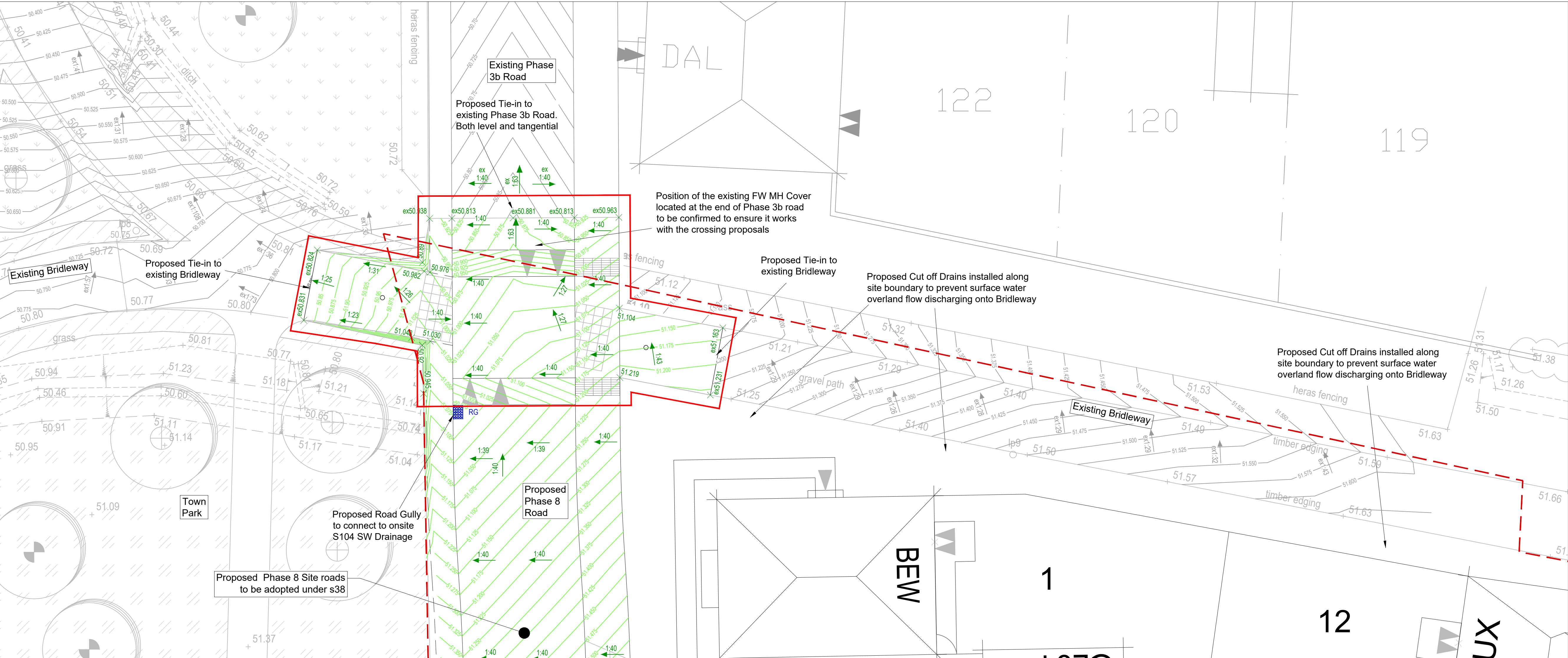
PROPOSED LEVELS PLAN SCALE 1:100
