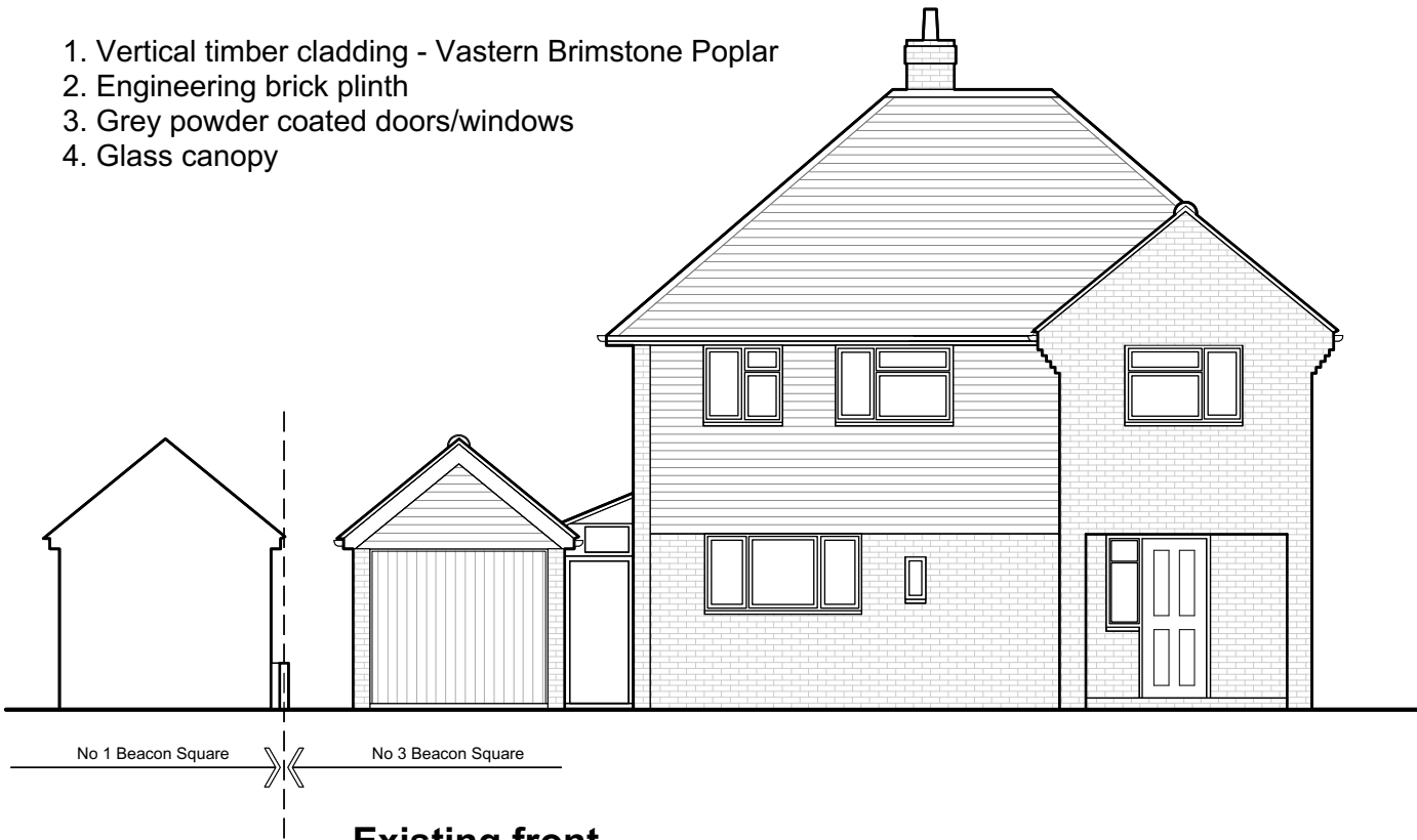
Existing front (north) elevation
