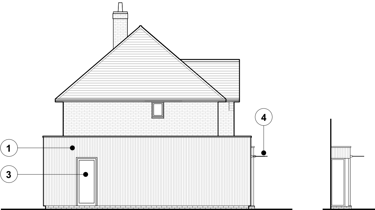
Proposed side (east) elevation
