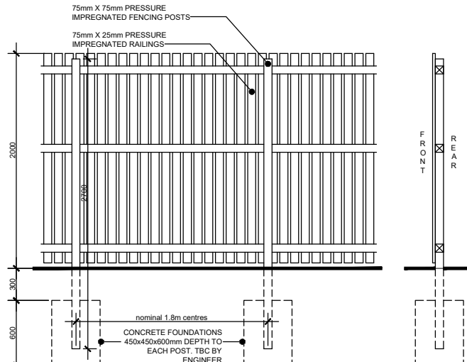
2000mm High Close Boarded Acoustic Timber Fence
