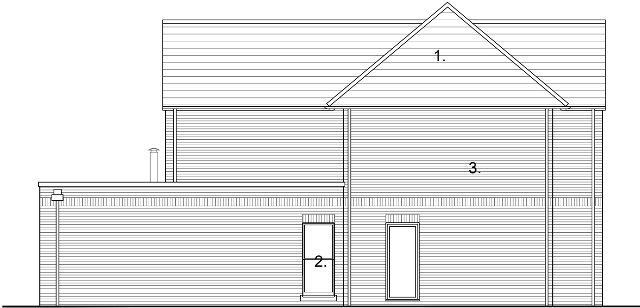
West Elevation
