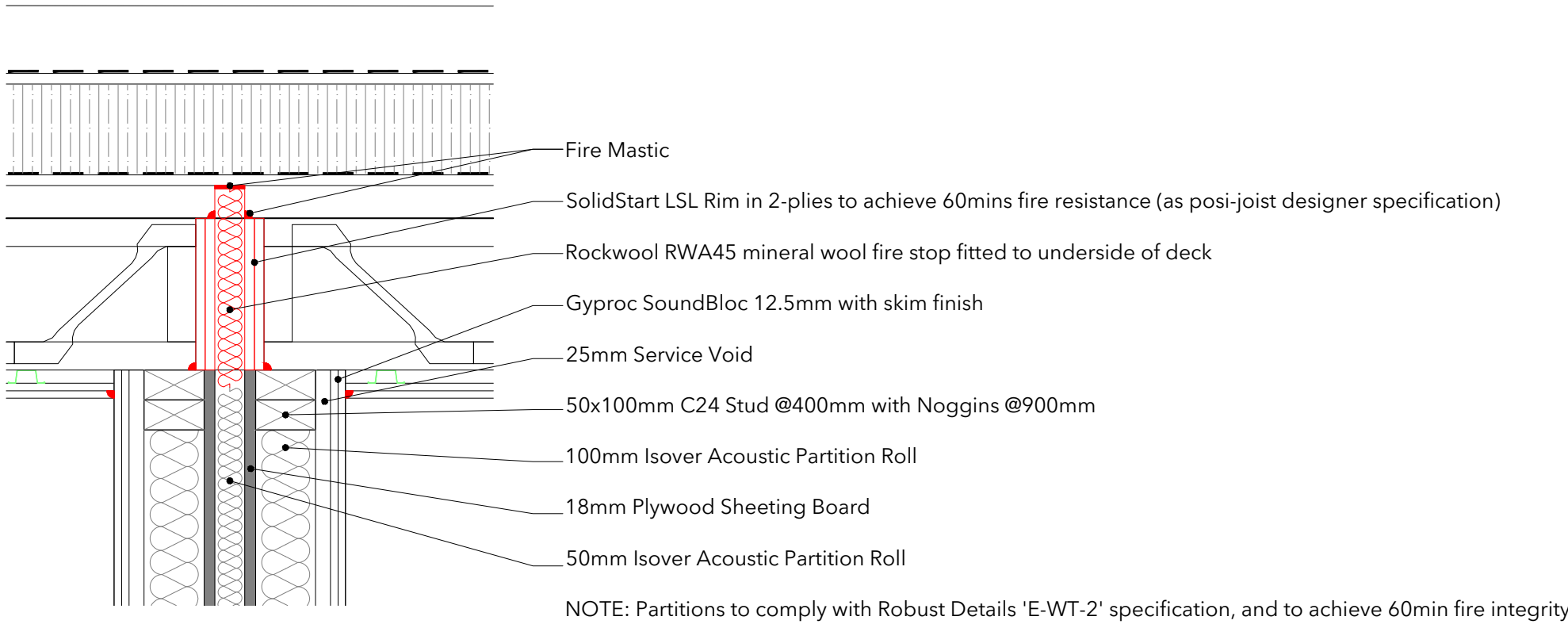
Detail A - Party Wall (loadbearing)
