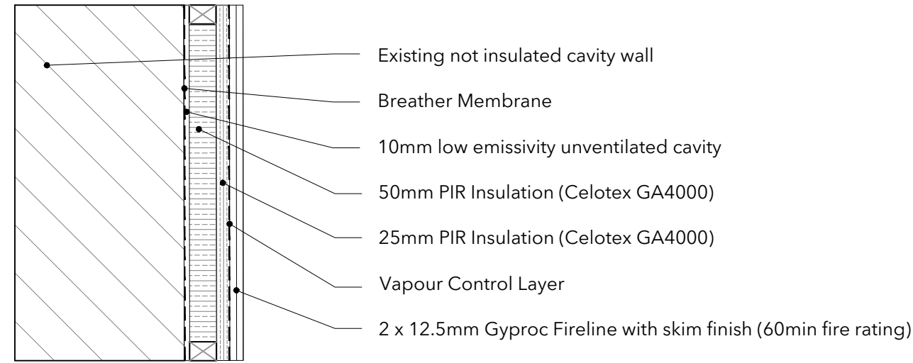
Detail B - Wall Upgrade
