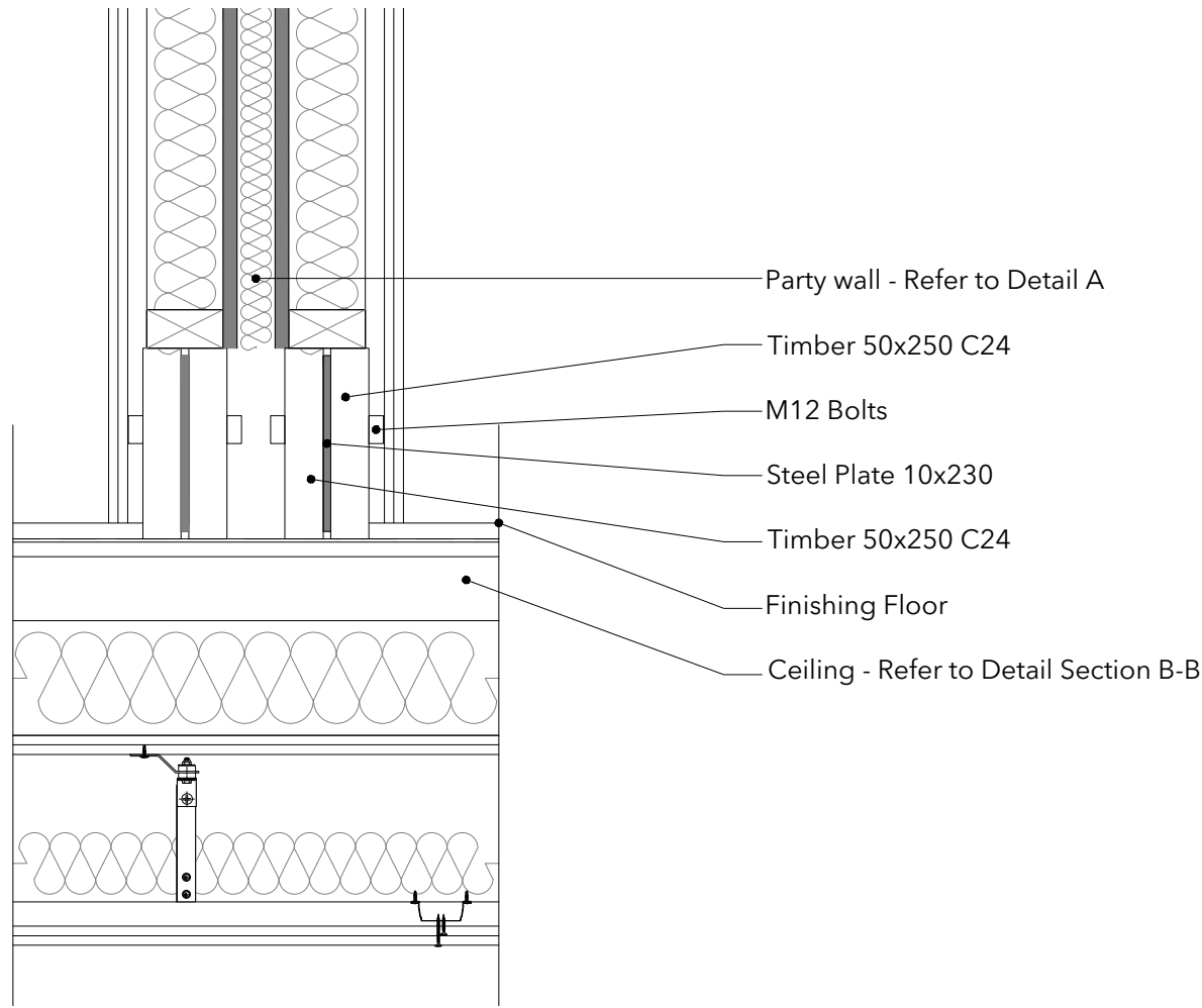
Detail C - Part Wall
