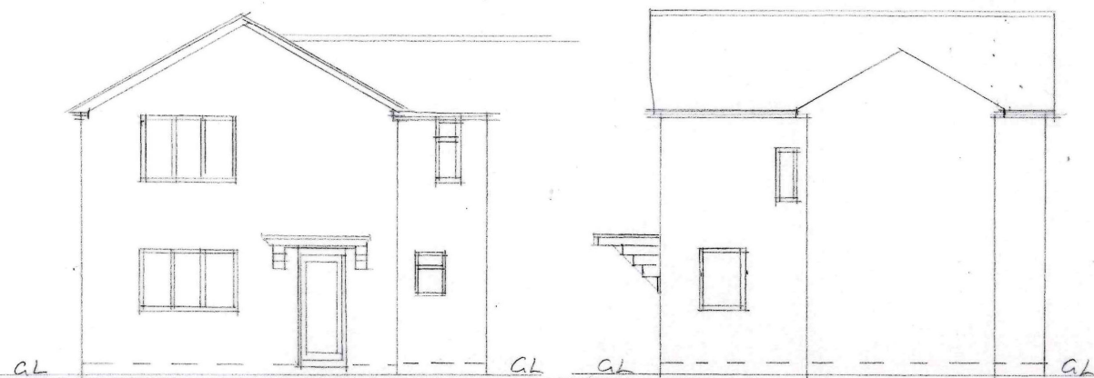
EXG FRONT ELEVATION
