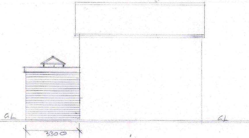
SIDE ELEVATION
