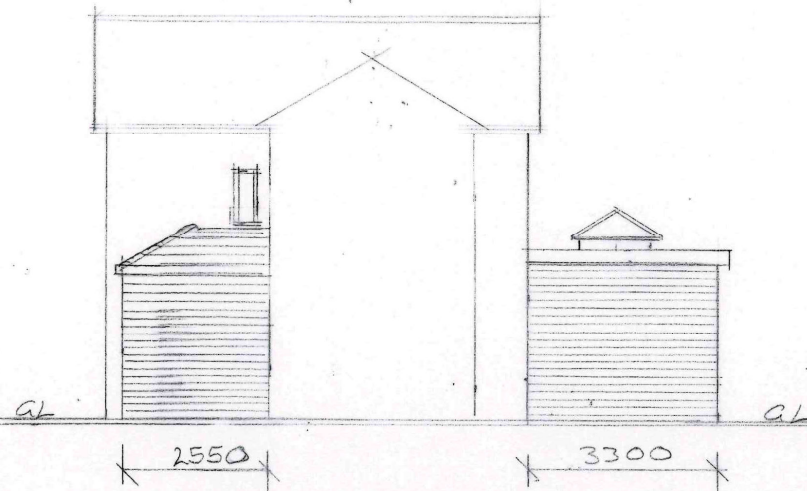
SIDE ELEVATION
