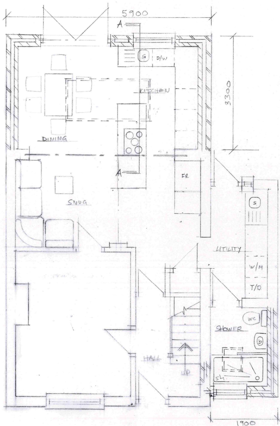
GROUND FLOOR PLAN 1:50@A3
